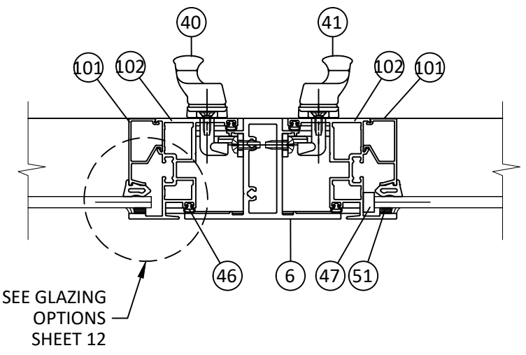
AQ 18 HORIZONTAL SECTION MEETING STILE "INSWING"
