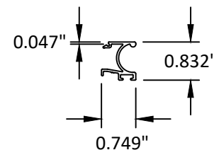
100 VENT GLASS STOP WITH PULL
