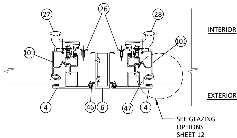
AJ HORIZONTAL SECTION 16 MEETING STILE "OUTSWING"
