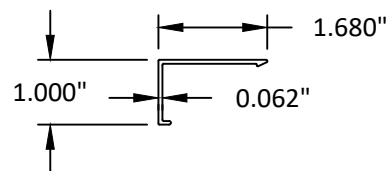
69 1" X 1 11/16" COVER
