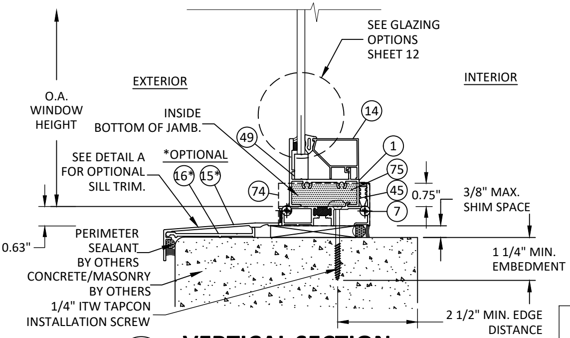
A 7 VERTICAL SECTION FIXED SILL - CONCRETE/MASONRY SILL FLASHING - TYP. "FIXED"
