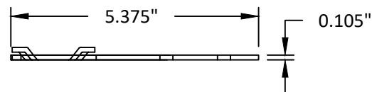
98 TWIST ANCHOR
