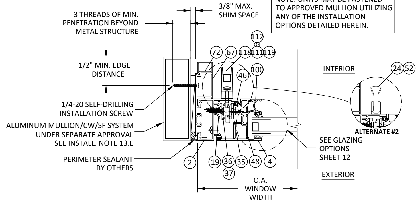
L 9 HORIZONTAL SECTION VENT JAMB - MULL TUBE FRAME STRAP ANCHOR - TYP. "OUTSWING" ALTERNATE #1
