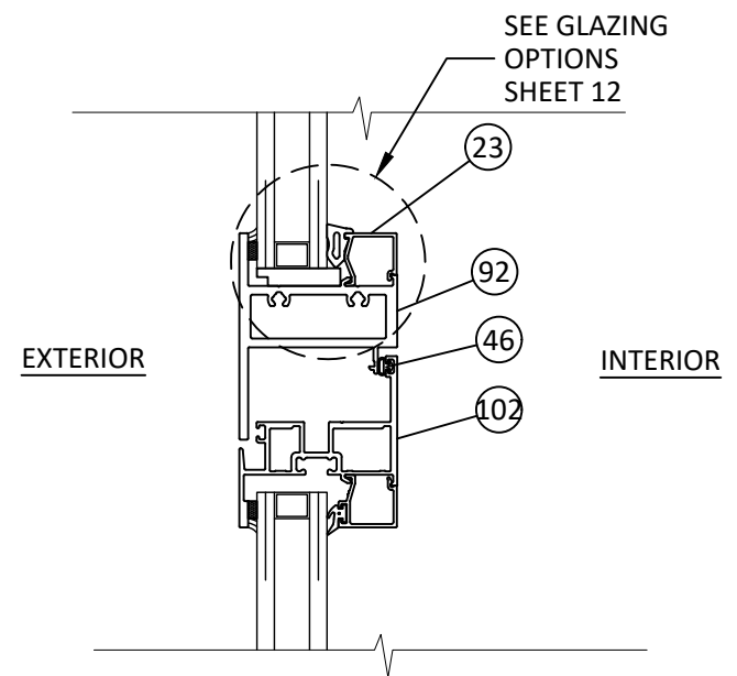
AR 18 VERTICAL SECTION INTEGRAL MULLION-TYP. FIXED OVER CASEMENT "INSWING"
